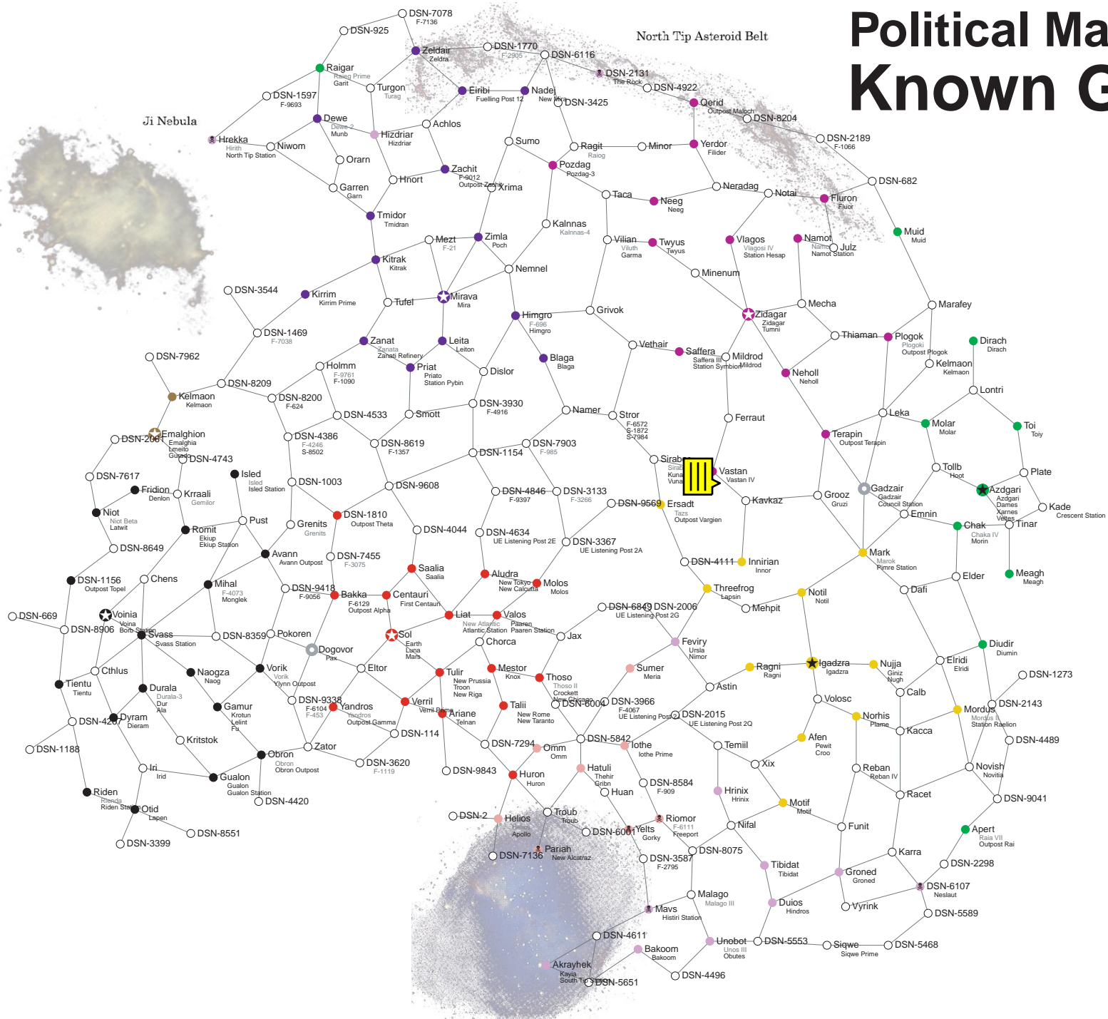
Proxima Nebula
